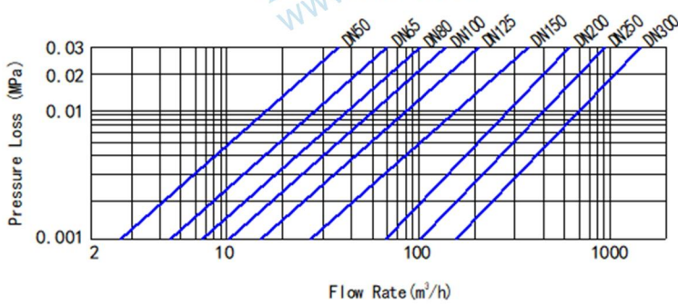
Pressure Loss Curve
